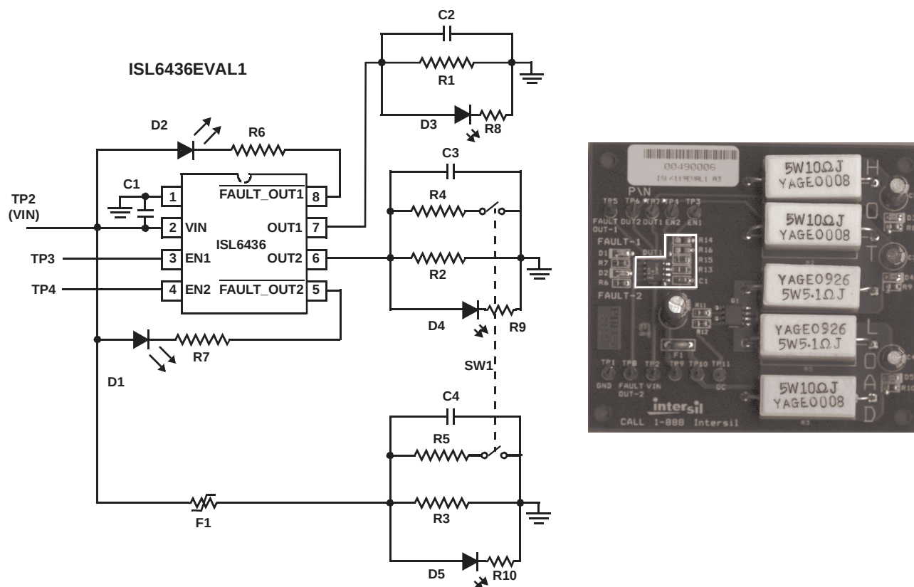
FIGURE 19. ISL6436EVAL1 BOARD SCHEMATIC AND PHOTOGRAPH
