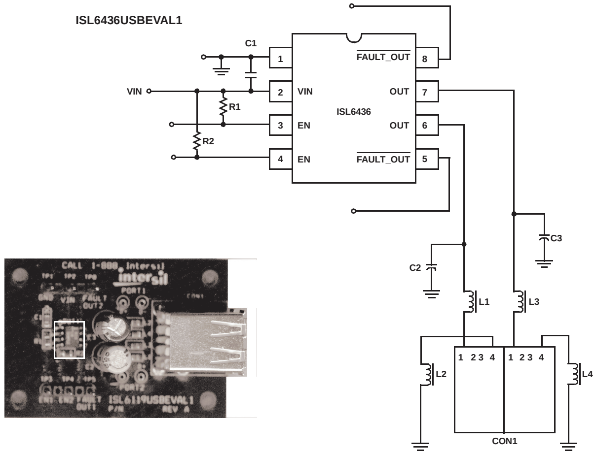
FIGURE 20. ISL6436USBEVAL BOARD
