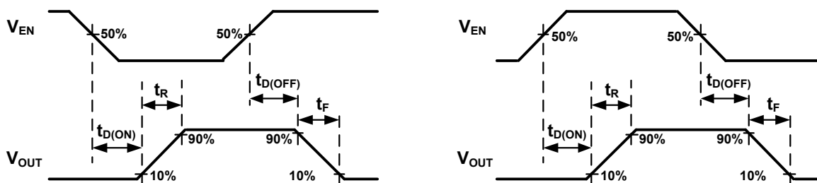
Figure 1. Voltage Waveforms: AP22652/52A (Left), AP22653/53A (Right)
