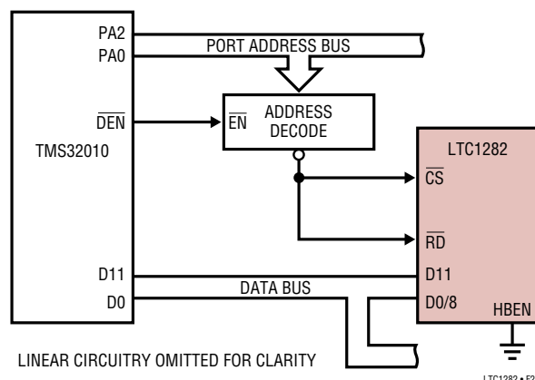
Figure 23. TMS32010 Interface
