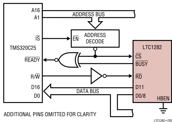
Figure 20. TMS320C25 Interface
