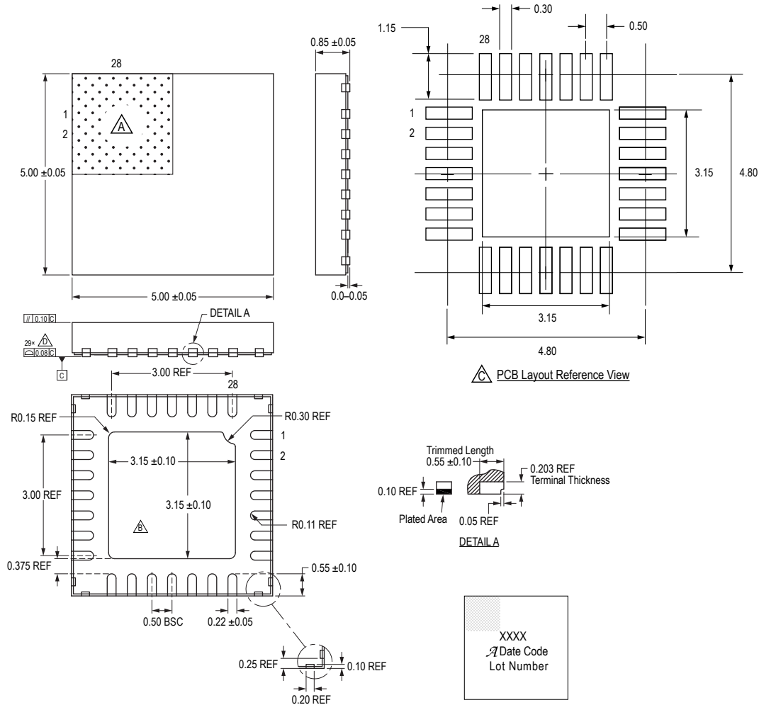
Figure 7: Package ET, 28-Pin QFN with Exposed Thermal Pad and Wettable Flank
