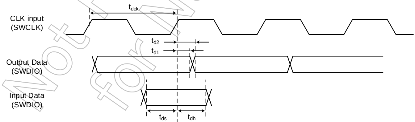
Figure 7.6 SWD waveform
