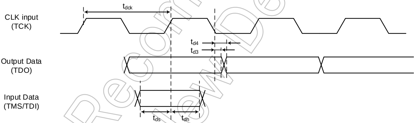
Figure 7.7 JTAG waveform
