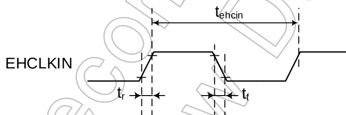
Figure 7.10 External clock input waveform
