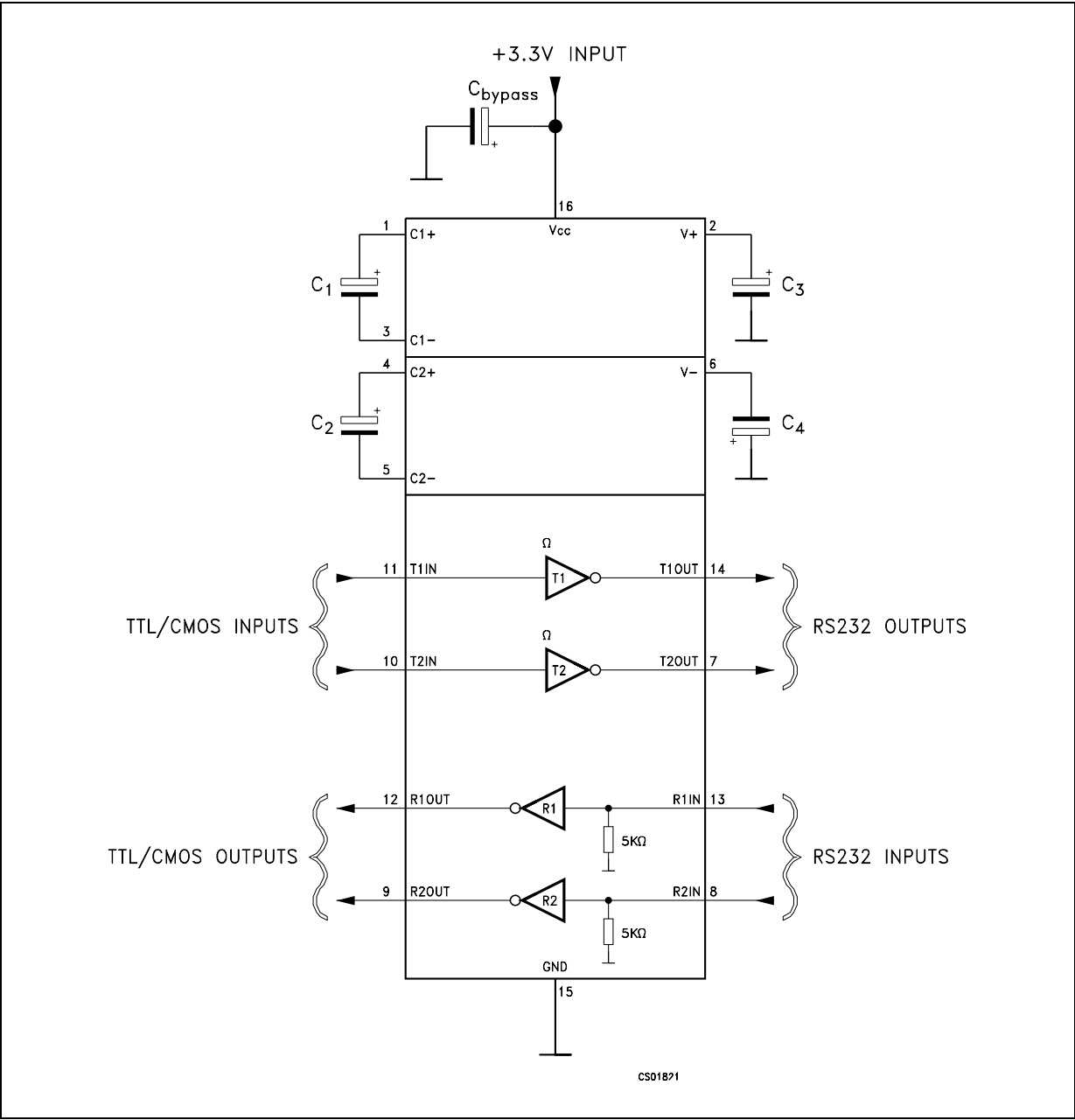
Figure 3. Application circuits
