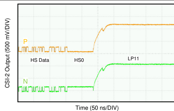
Figure 8-11. CSI-2 End of Transmission (EoT)
