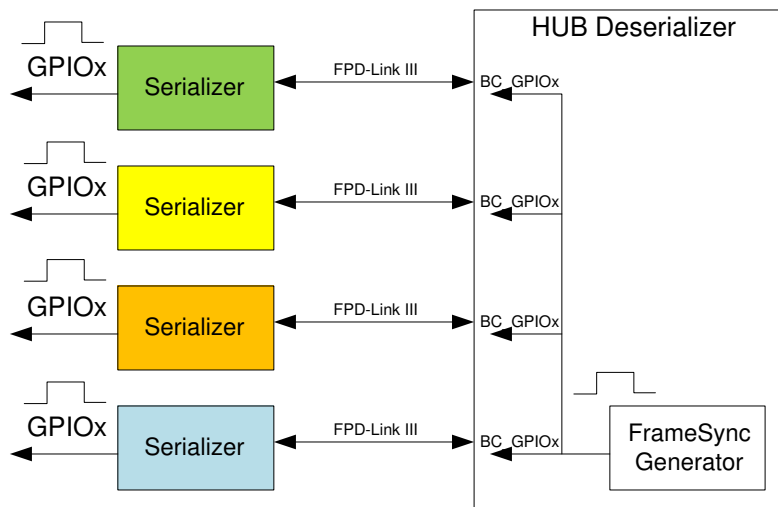
Figure 7-14. Internal FrameSync
