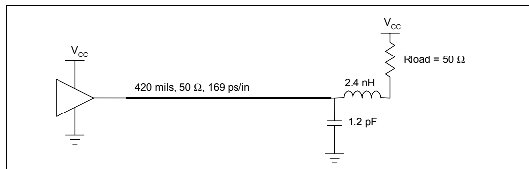
Figure 2-7. Test Circuit
