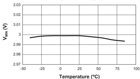
Preconditioning Voltage Threshold vs. Temperature ( R_{SET} = 8.06k\Omega )
