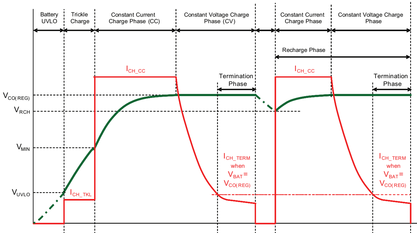
Figure 1: Current vs. Voltage Profile During Charging Phases.
