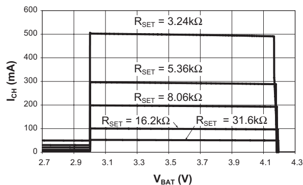
Charging Current vs. Battery Voltage ( V_{ADP} = 5V )
