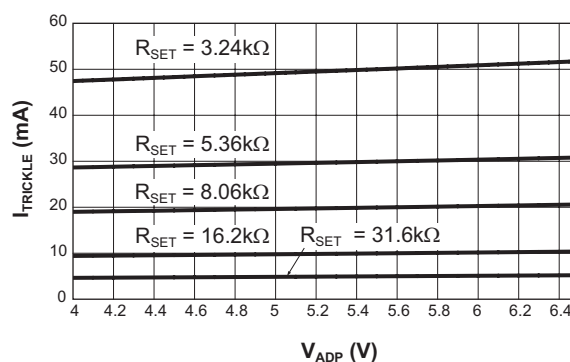
Preconditioning Charge Current vs. Adapter Voltage
