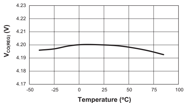
Constant Output Charge Voltage Regulation vs. Temperature ( R_{SET} = 8.06k\Omega )
