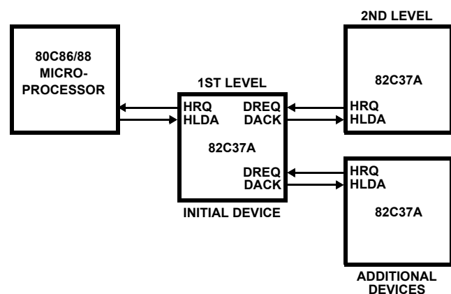
FIGURE 3. CASCADED 82C37As
