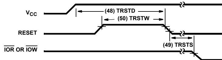
FIGURE 14. RESET
