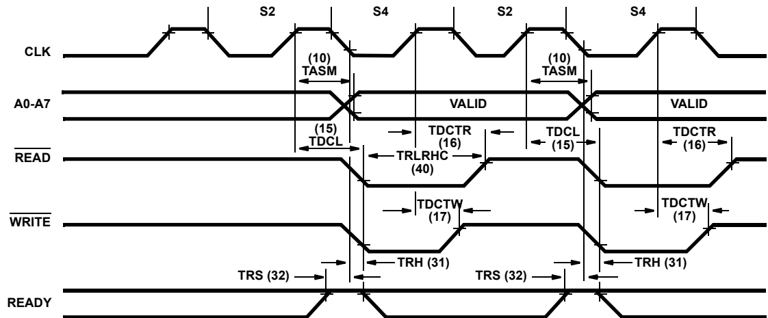
FIGURE 13. COMPRESSED TRANSFER
