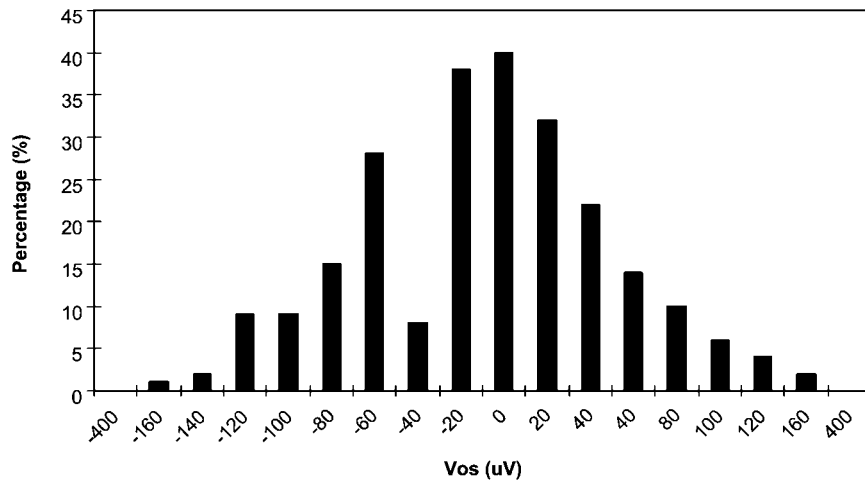
Offset Voltage Distribution V_{CC} = \pm 20V
