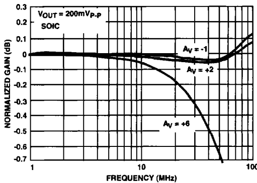
FIGURE 14. GAIN FLATNESS
