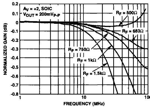
FIGURE 15. GAIN FLATNESS vs FEEDBACK RESISTOR
