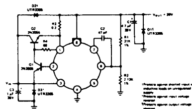
1.0A Regulator with Protective Diodes
