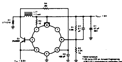
Switching Regulator
