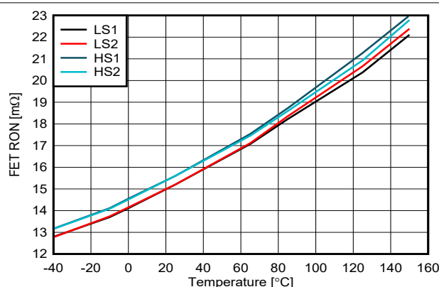
Figure 7-12. R_{HS\_ON} & R_{LS\_ON} for VQFN-HR(16) vs Temperature at V_{VM} = 13.5\text{ V}
