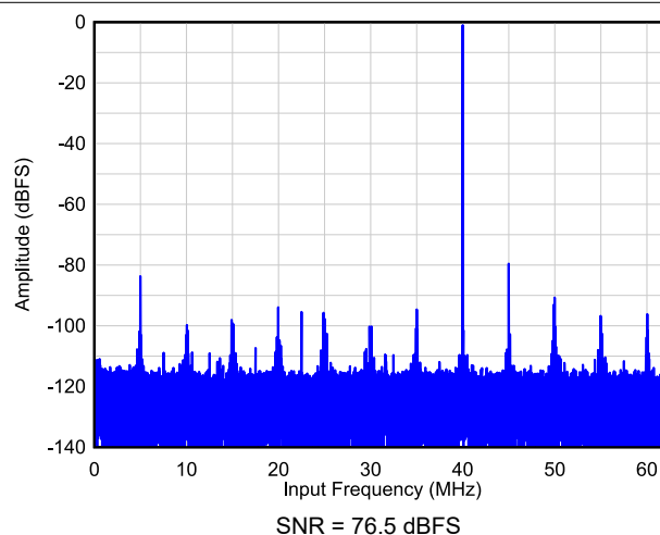
Figure 6-4. Single Tone FFT at F_{IN} = 40\text{ MHz}
