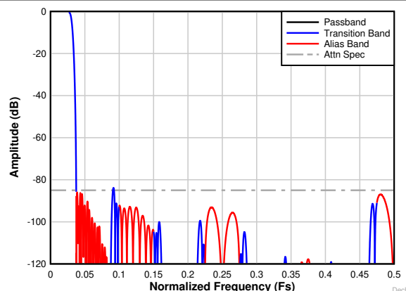
Figure 8-26. Decimation by 16 complex frequency response
