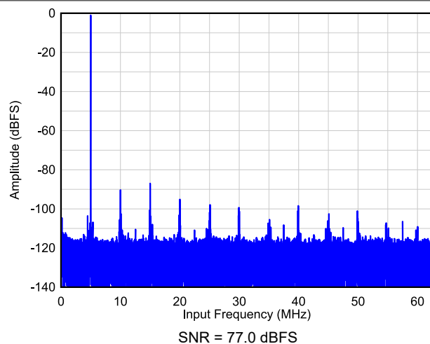
Figure 6-1. Single Tone FFT at F_{IN} = 5\text{ MHz}
