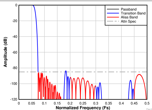
Figure 8-24. Decimation by 8 complex frequency response
