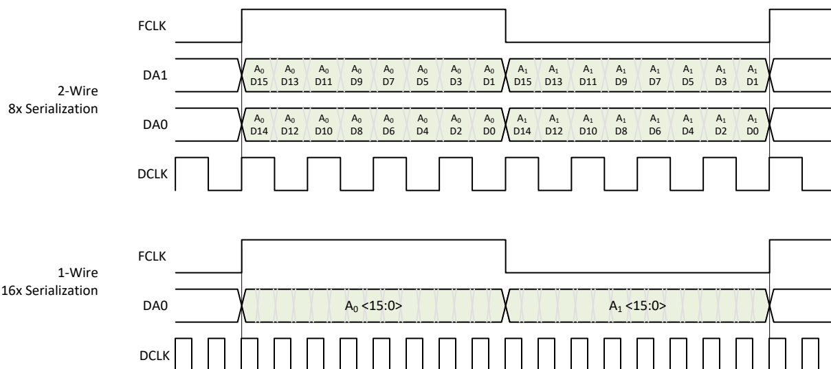
Figure 8-32. Output Data Format in Real Decimation
