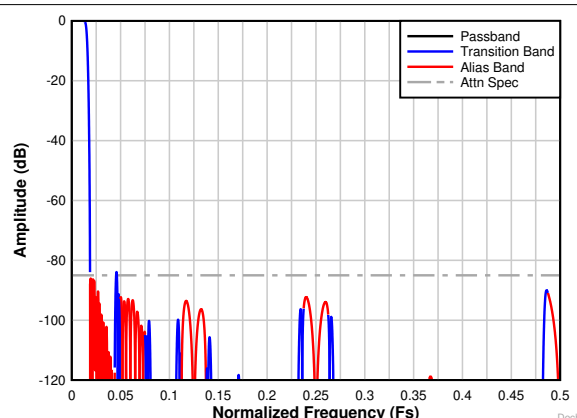
Figure 8-28. Decimation by 32 complex frequency response
