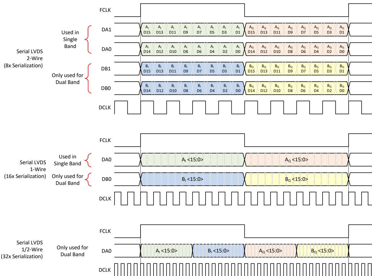
Figure 8-31. Output Data Format in Complex Decimation
