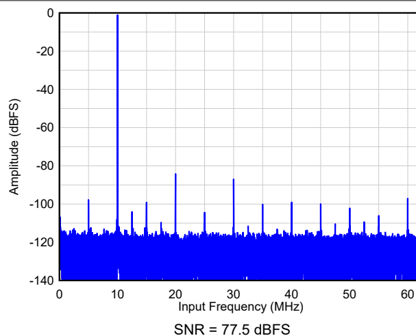
Figure 6-2. Single Tone FFT at F_{IN} = 10\text{ MHz}
