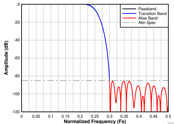
Figure 8-20. Decimation by 2 complex frequency response
