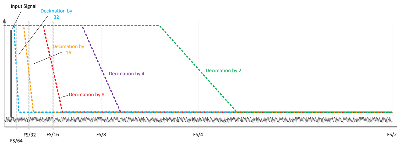
Figure 8-17. Real decimation illustration
