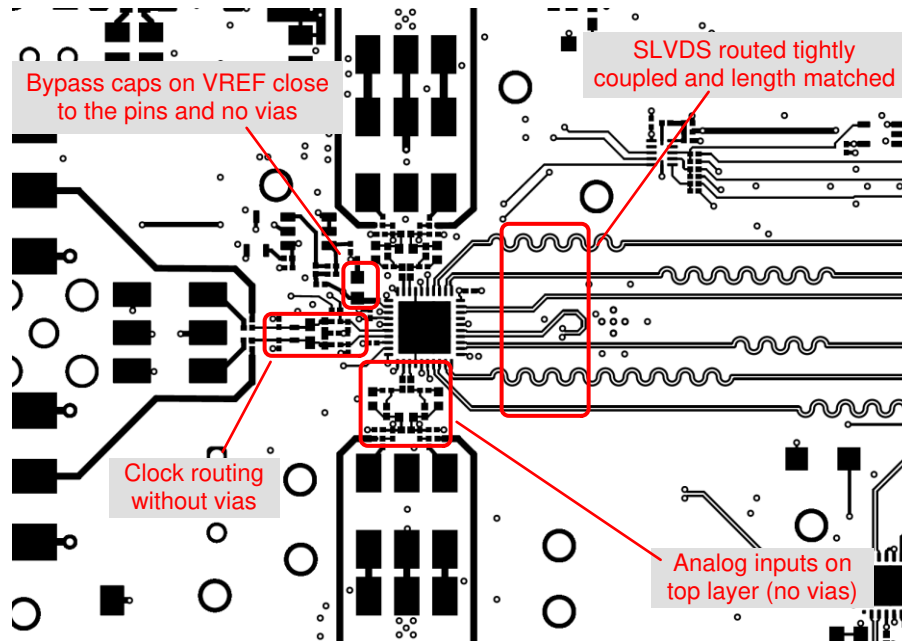
Figure 9-10. Layout example: top layer of ADC3564 EVM
