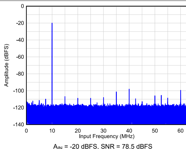
Figure 6-3. Single Tone FFT at F_{IN} = 10\text{ MHz}
