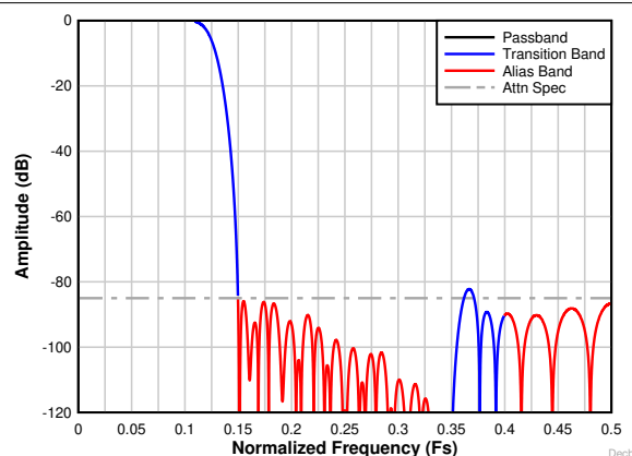
Figure 8-22. Decimation by 4 complex frequency response
