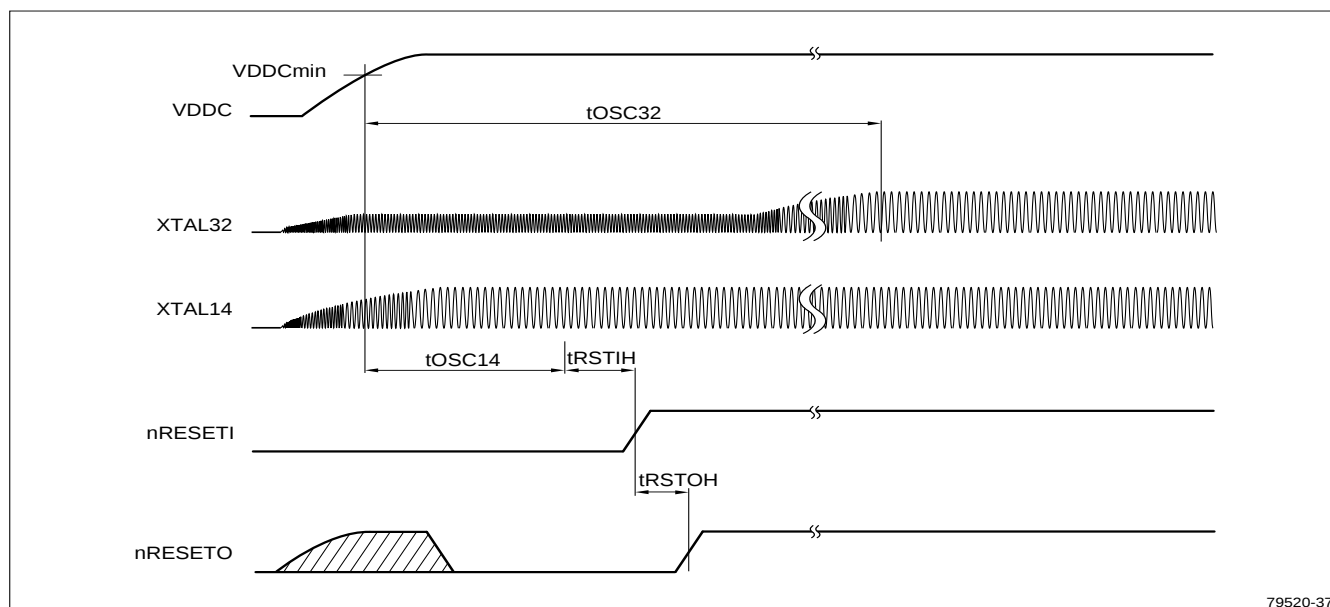
Figure 29. PLL Start-up
