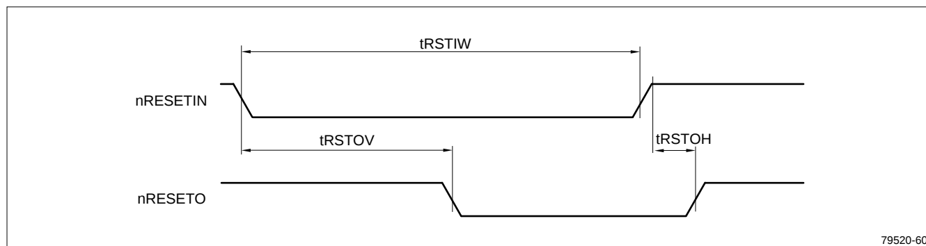
Figure 30. External Reset
