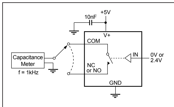
Figure 5. Channel-Off Capacitance
