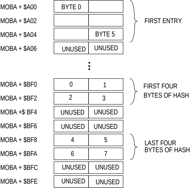
Figure 4-6. AR Memory Map - Hash Mode
