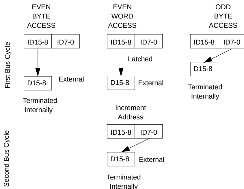
Figure 2-3. 16-bit Internal to 8-bit External Write
