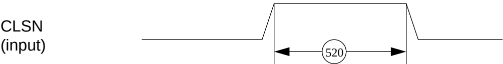
Figure 8-4. Ethernet Collision Timing
