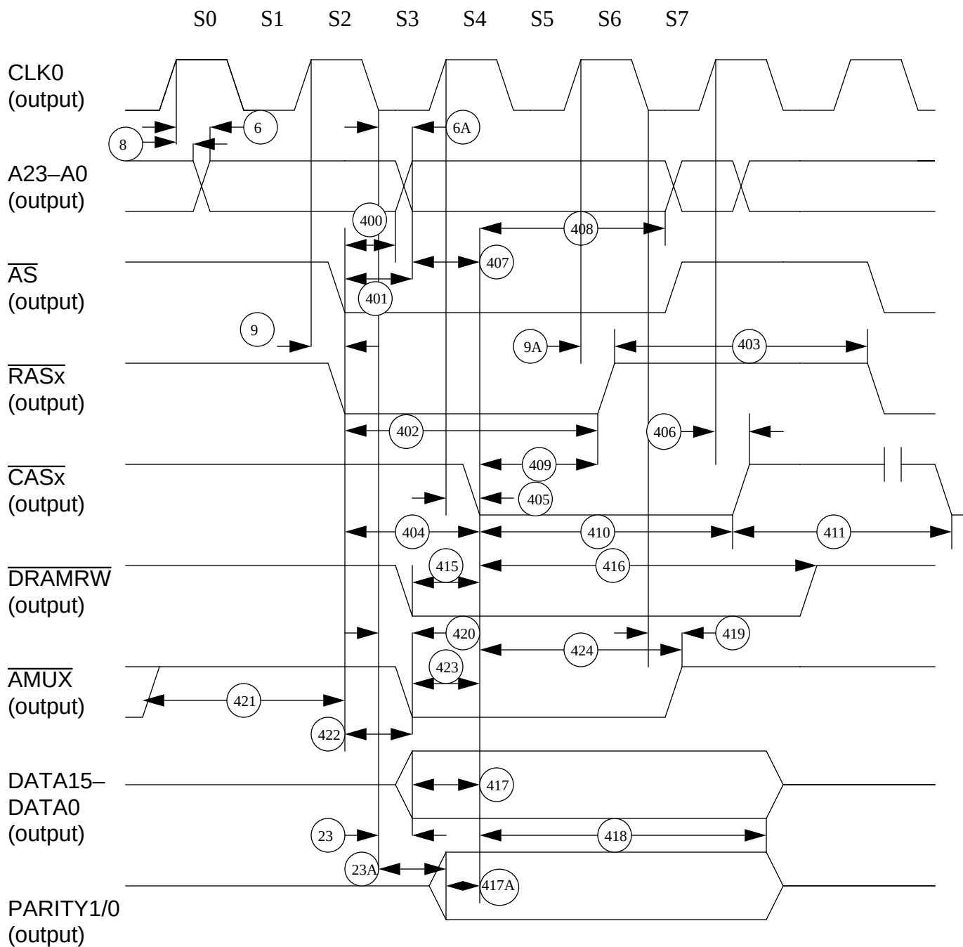
Figure 8-2. DRAM Write Cycle
