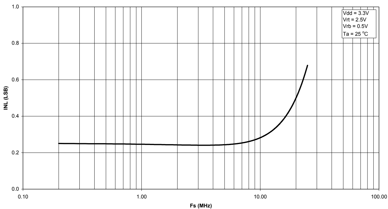
Graph 4. Best Fit INL vs. Sampling Frequency
