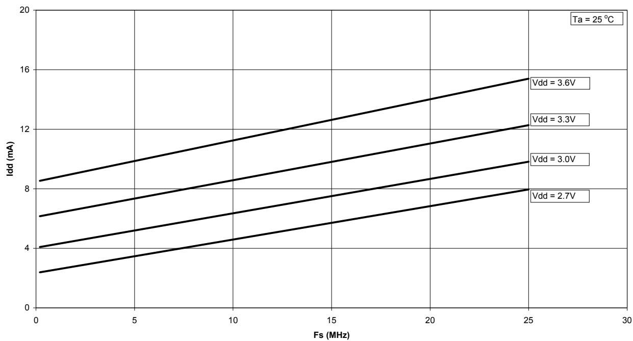
Graph 5. IDD vs. Sampling Frequency
