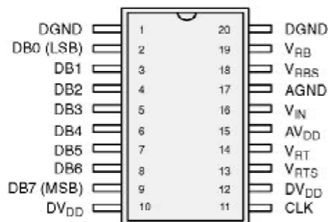
20-Pin SOIC (Jedec, 300 MIL) - D20
