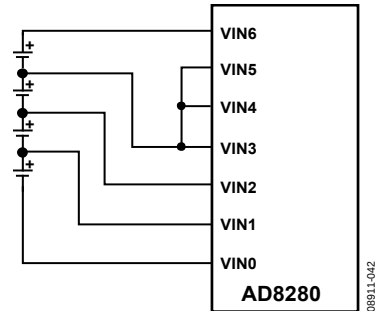
Figure 48. Four-Cell Connections for the AD8280
