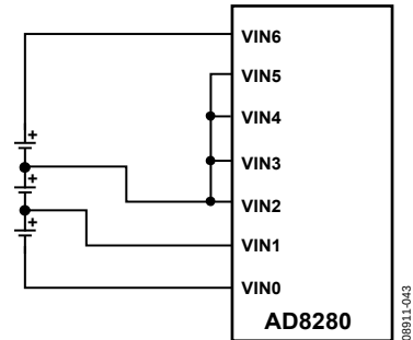
Figure 49. Three-Cell Connections for the AD8280
