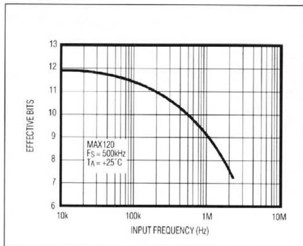
Figure 23. Effective Bits vs. Input Frequency
