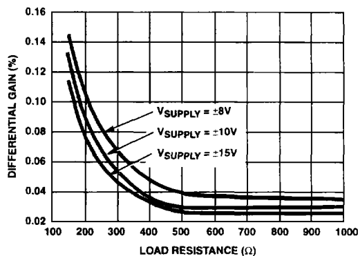
FIGURE 18. DIFFERENTIAL GAIN vs LOAD RESISTANCE
