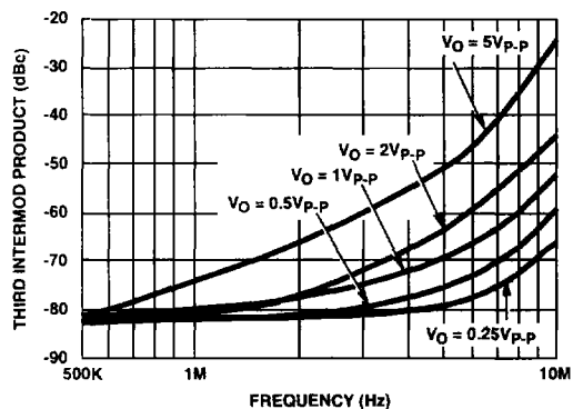
FIGURE 17. INTERMODULATION DISTORTION vs FREQUENCY (TWO TONE)
