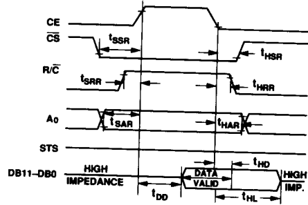
Figure 2. Read Timing
