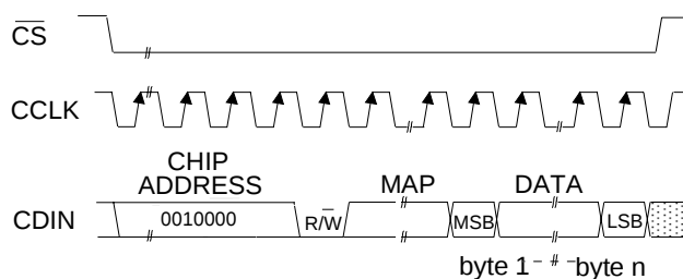
Figure 7. SPI Mode Control Port Formatting
