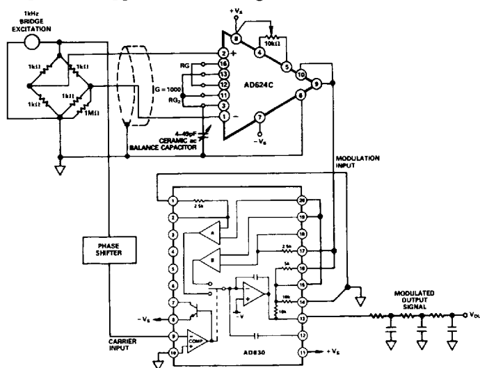
Figure 45. AC Bridge
