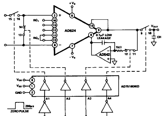
Figure 42. Auto-Zero Circuit
