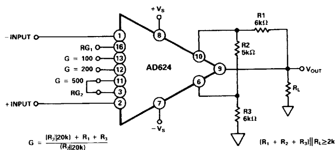
Figure 30. Gain of 2500
