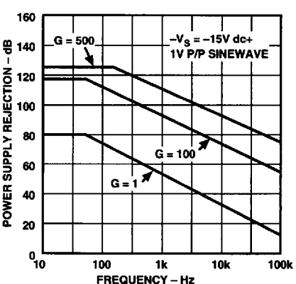
Figure 12. Positive PSRR vs. Frequency
