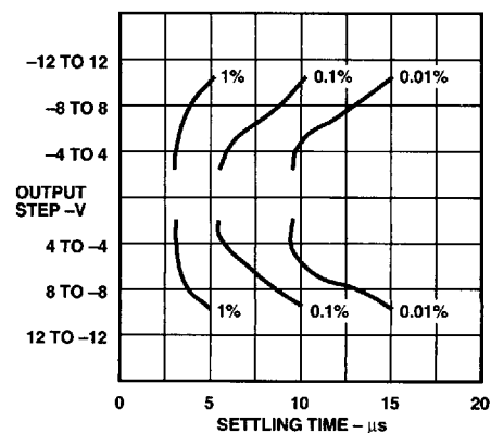
Figure 18. Settling Time, G = 1
