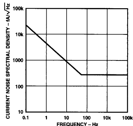
Figure 15. Input Current Noise
