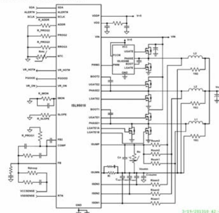
Simplified Application Circuit
