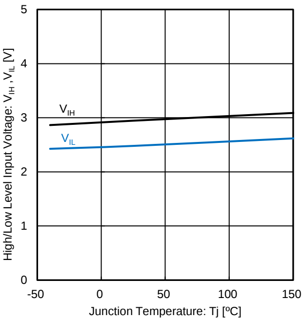
Figure 13. High/Low Level Input Voltage vs Junction Temperature
