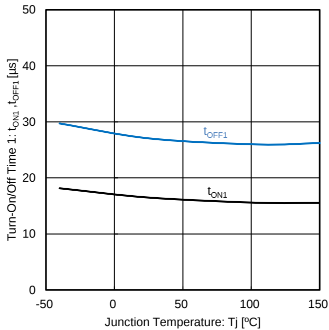
Figure 25. Turn-On/Off Time 1 vs Junction Temperature
