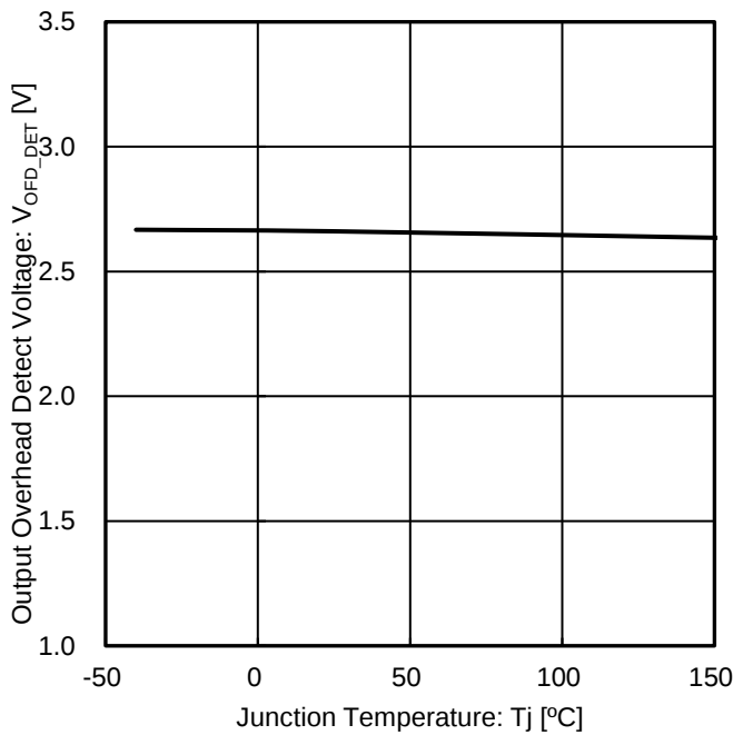
Figure 41. Output Overhead Detect Voltage vs Junction Temperature
