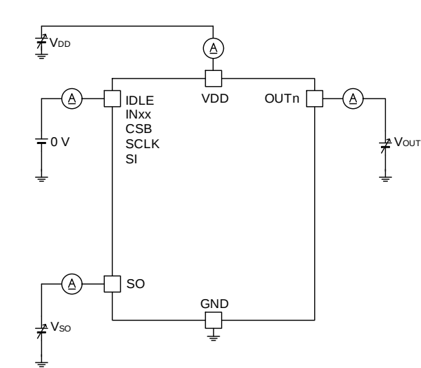
Figure 47. VDD Standby Current Low Level Input Current 1, 2 Output Leakage Current Serial Out Output Leakage Current
