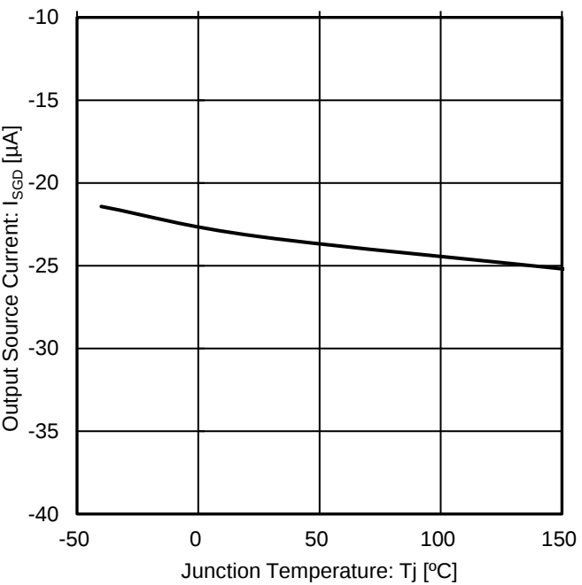
Figure 45. Output Source Current vs Junction Temperature
