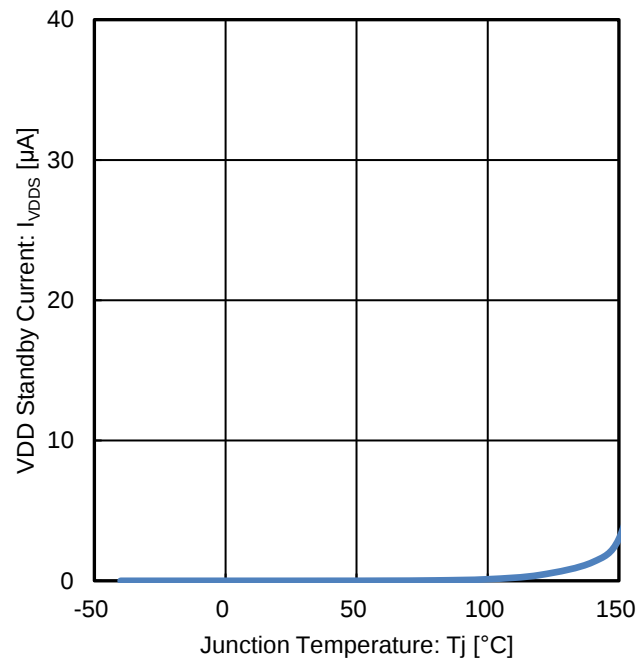
Figure 9. VDD Standby Current vs Junction Temperature
