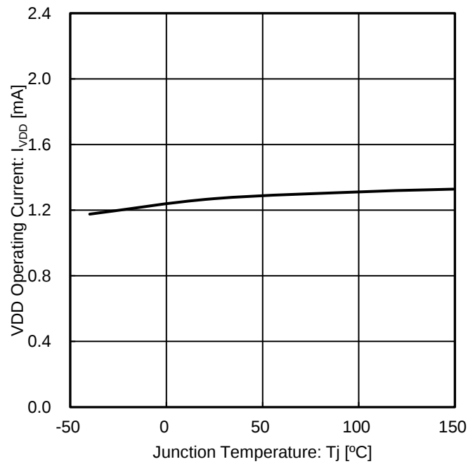
Figure 11. VDD Operating Current vs Junction Temperature
