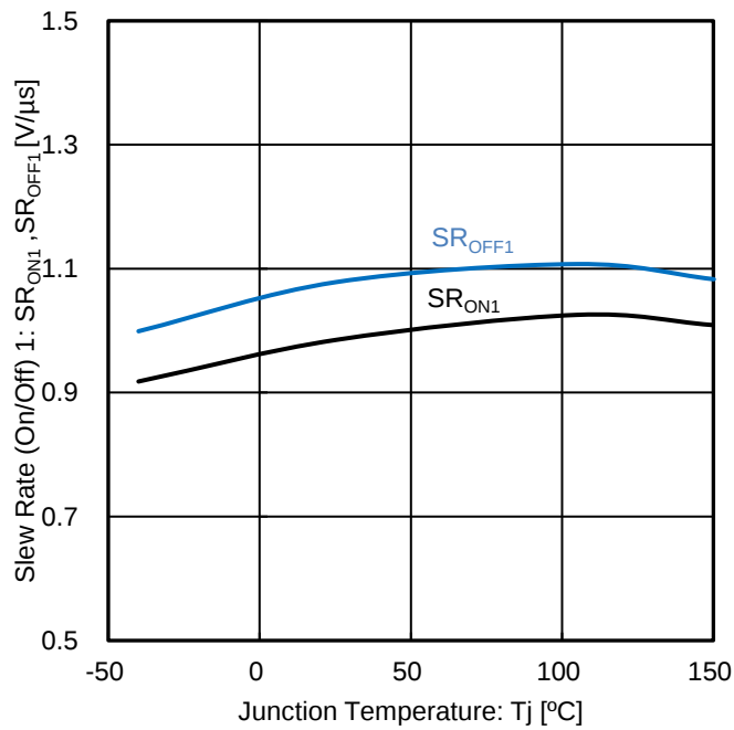
Figure 27. Slew Rate (On/Off) 1 vs Junction Temperature
