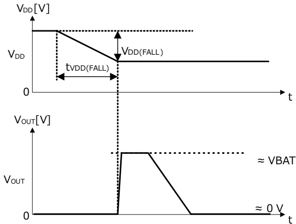
Figure 55. Output OFF operation when power supply fluctuates sharply
