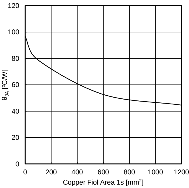
Figure 7. Thermal Resistance
