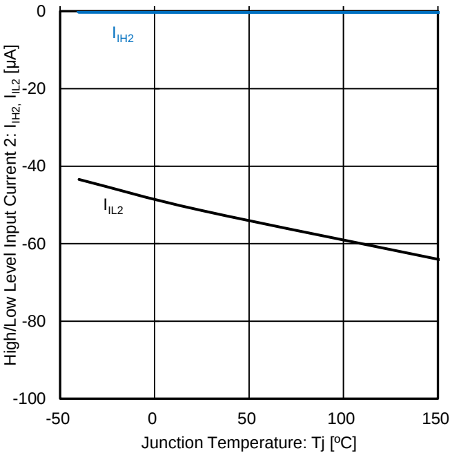
Figure 15. High/Low Level Input Current 2 vs Junction Temperature
