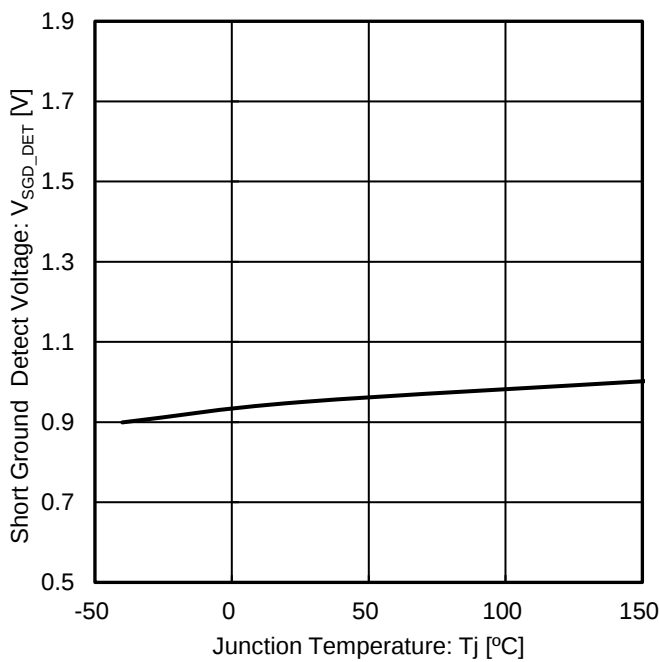
Figure 43. Short Ground Detect Voltage vs Junction Temperature
