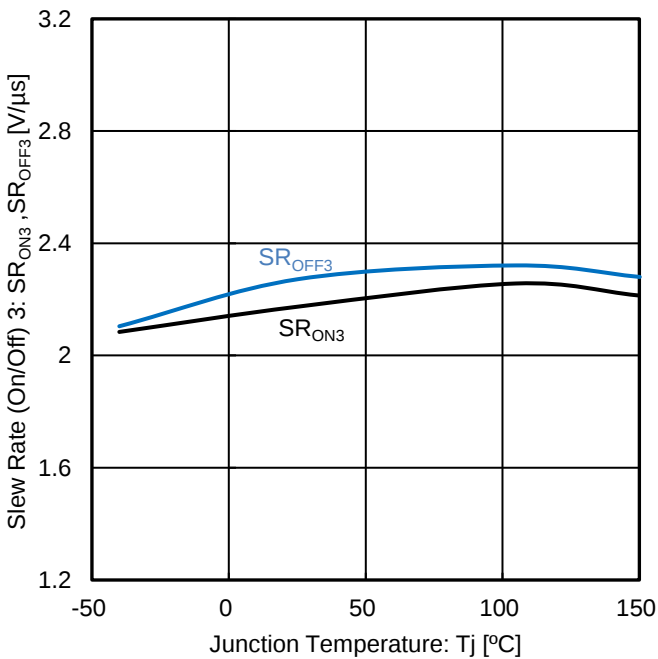
Figure 35. Slew Rate (On/Off) 3 vs Junction Temperature
