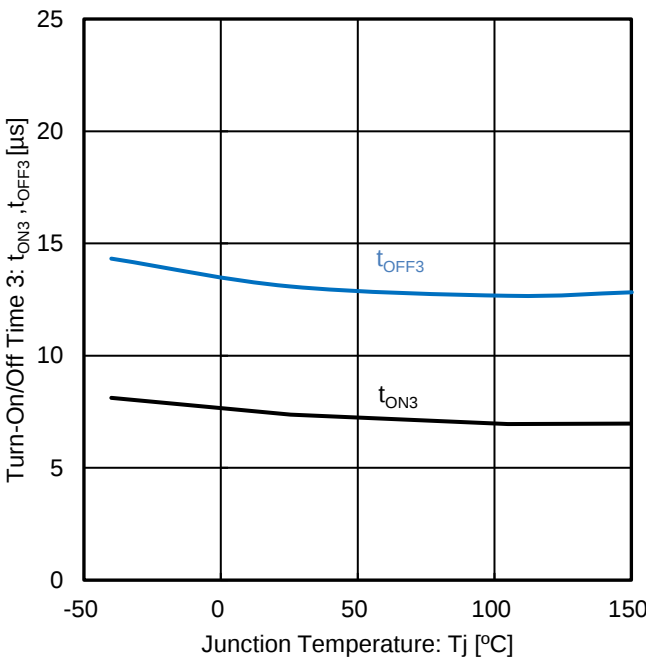
Figure 33. Turn-On/Off Time 3 vs Junction Temperature
