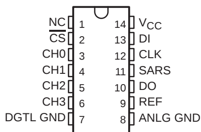
TLV0834 . . . D OR N PACKAGE (TOP VIEW)
