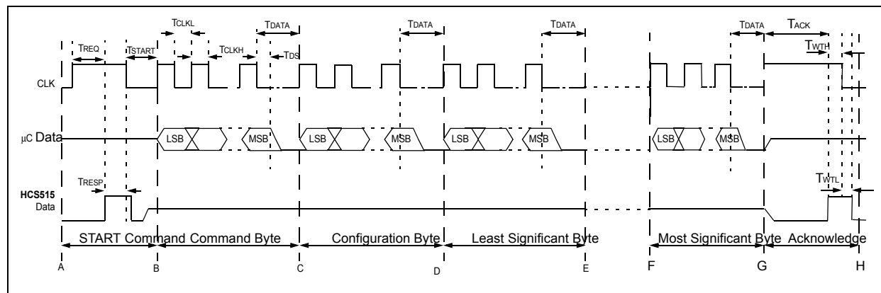
FIGURE 5-1: PROGRAMMING WAVEFORM
