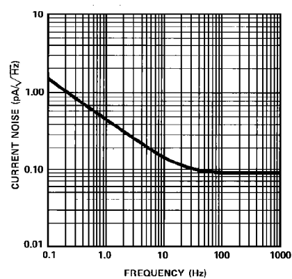
CURRENT NOISE DENSITY ( i_n ) vs FREQUENCY
