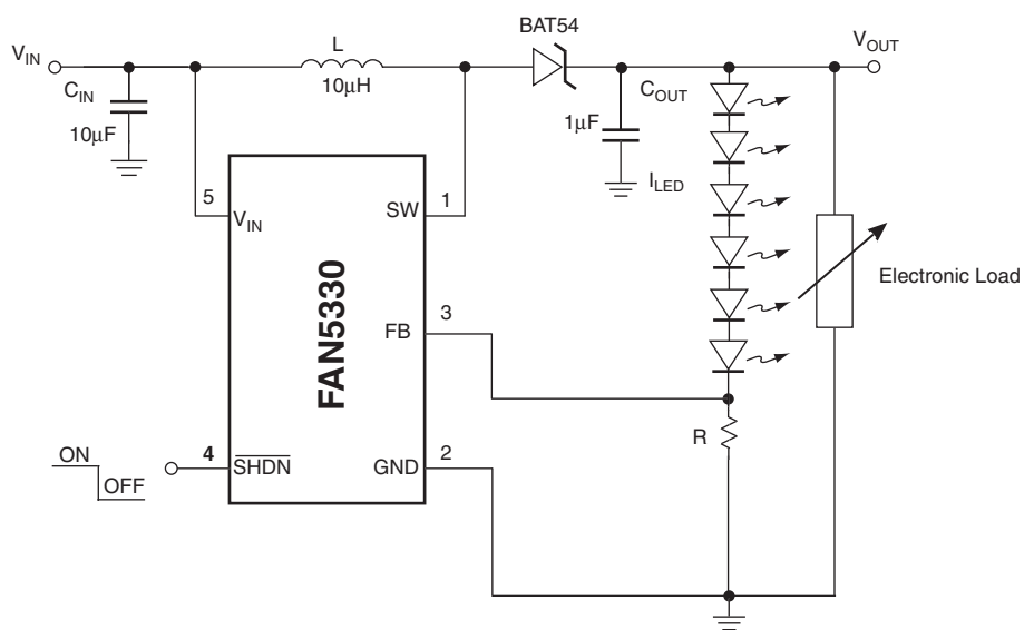
Figure 3. Test Circuit
