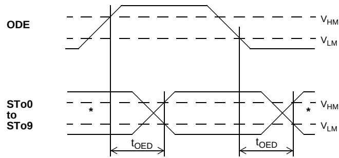
Figure 20 - Output Driver Enable for Streams at 4.096 and 8.192 Mb/s
