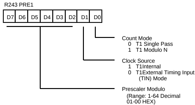
Figure 54. Prescaler 1 Register (F3 H : Write-Only)
