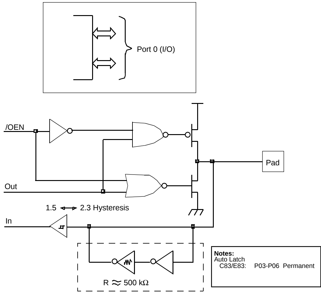
Figure 10. Port 0 Configuration
