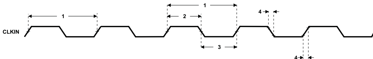
Figure 5-9. CLKIN Timing
