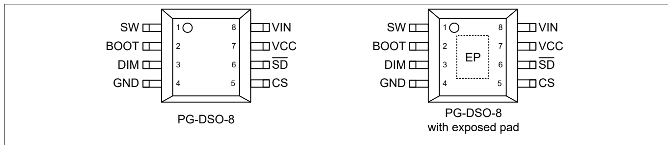
Figure 3 Pin-out
