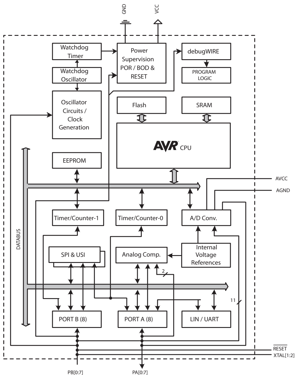
Figure 1-1. Block Diagram
