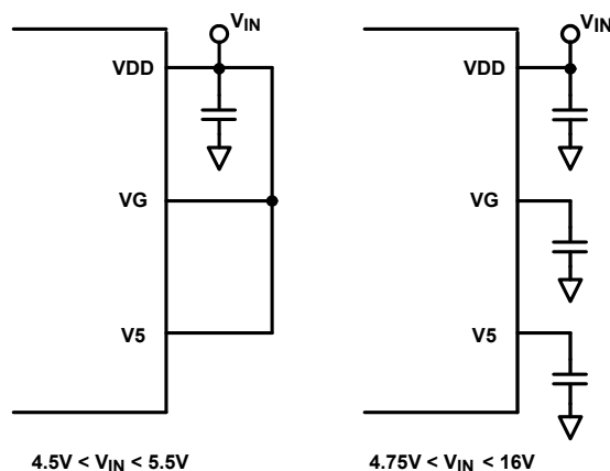
Figure 7. Supply Connections
