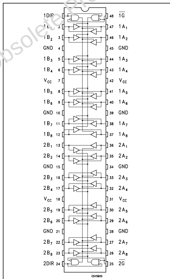
Figure 1: Pin Connection
