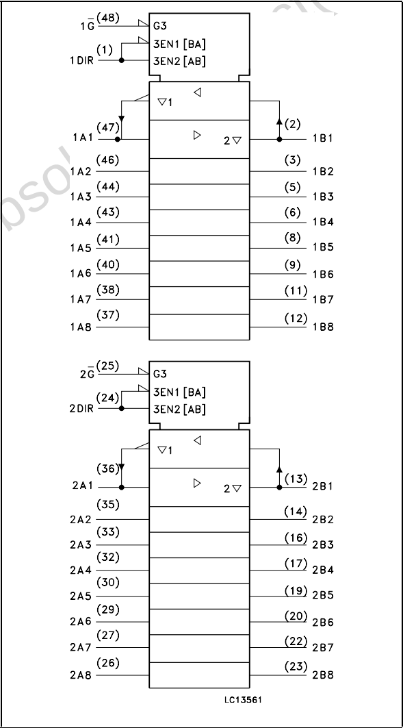
Figure 3: IEC Logic Symbols
