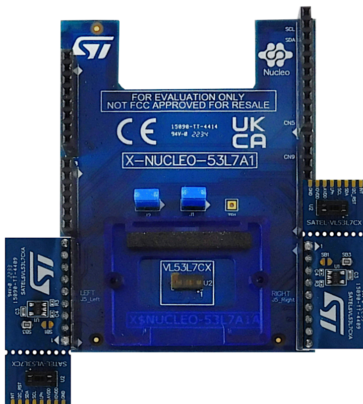
Figure 2. SATEL-VL53L7CX breakout boards connected to the X-NUCLEO-53L7A1 expansion board
