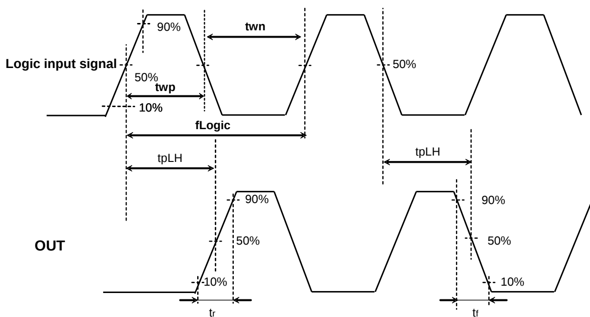
Figure 1 Logic input and switching characteristics of output transistors
