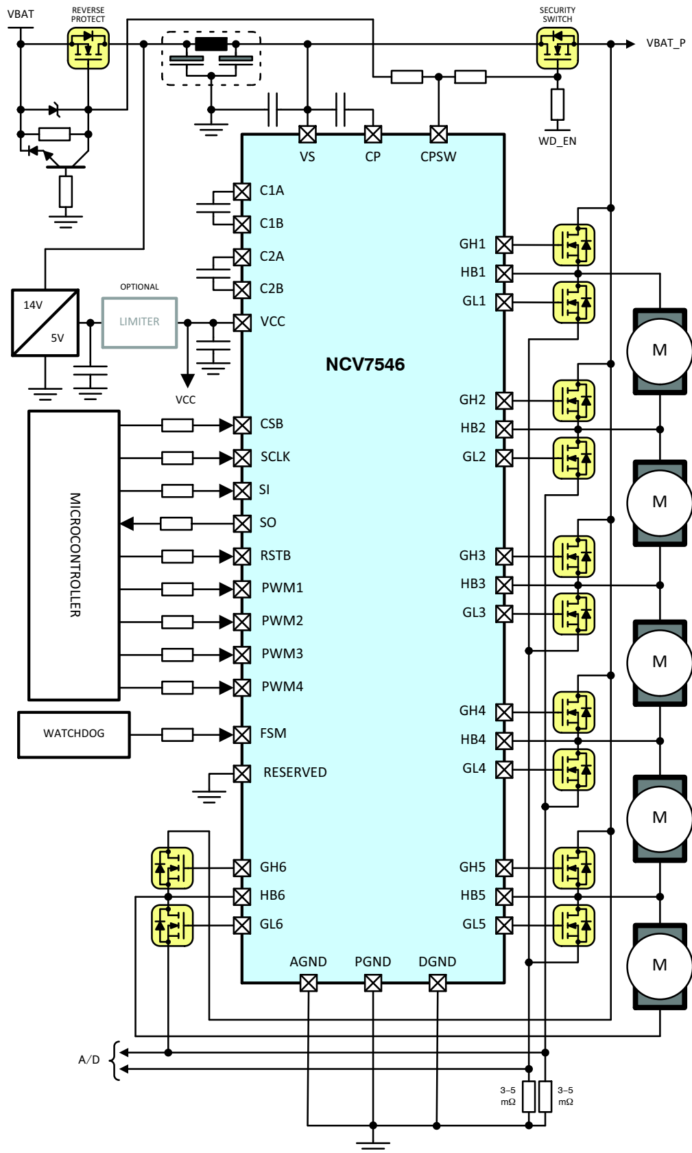
Figure 2. Application Diagram
