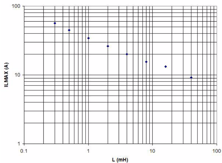
Figure 14. Maximum Turn-off Current Versus Inductive Load (Single Pulse for R_L = 0 and V_{PWR} = 12\text{ V} at T_J = 150\text{ }^{\circ}\text{C} Initial)
