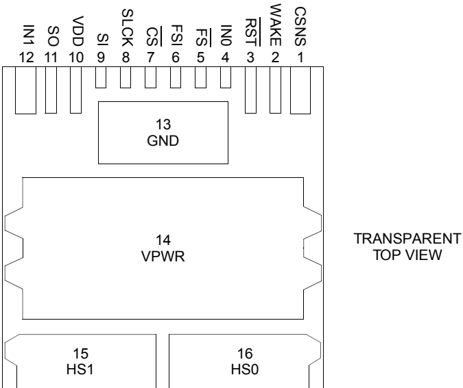
Figure 3. 34988 Pin Connections (Transparent Top View)
