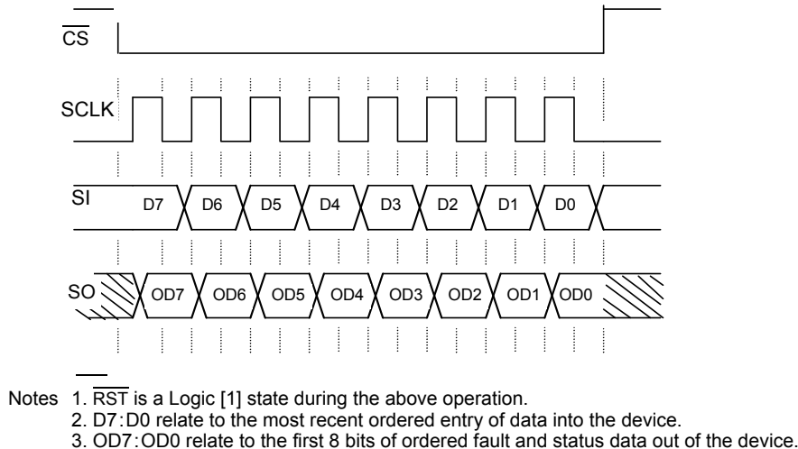
Figure 11. Single 8-Bit Word SPI Communication
