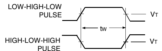
Pulse Width
