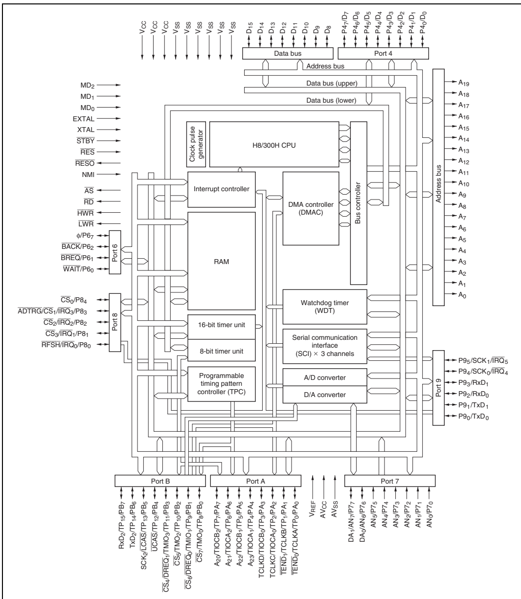
Figure 1.1 Block Diagram
