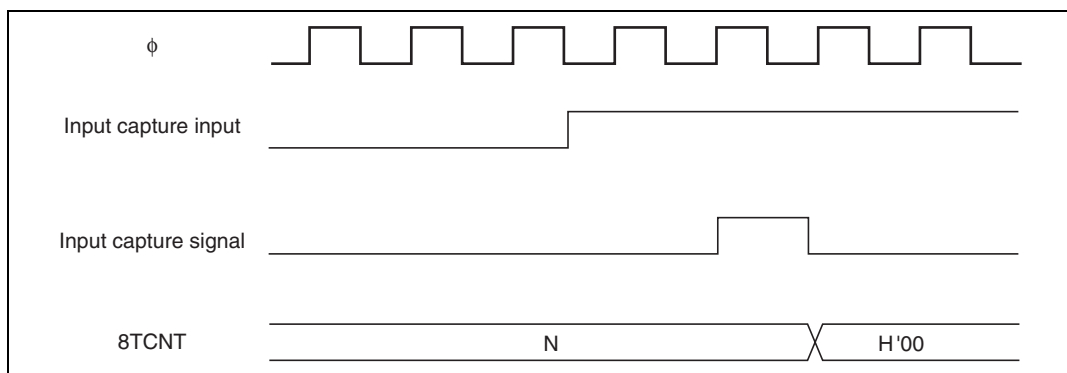
Figure 10.12 Timing of Clear by Input Capture
