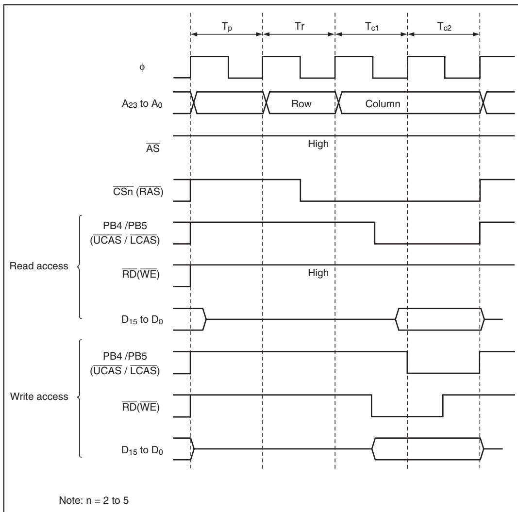
Figure 6.16 Basic Access Timing (CSEL = 0 in DRCRB)
