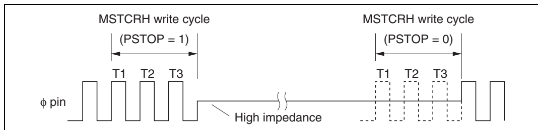
Figure 19.3 Starting and Stopping of System Clock Output
