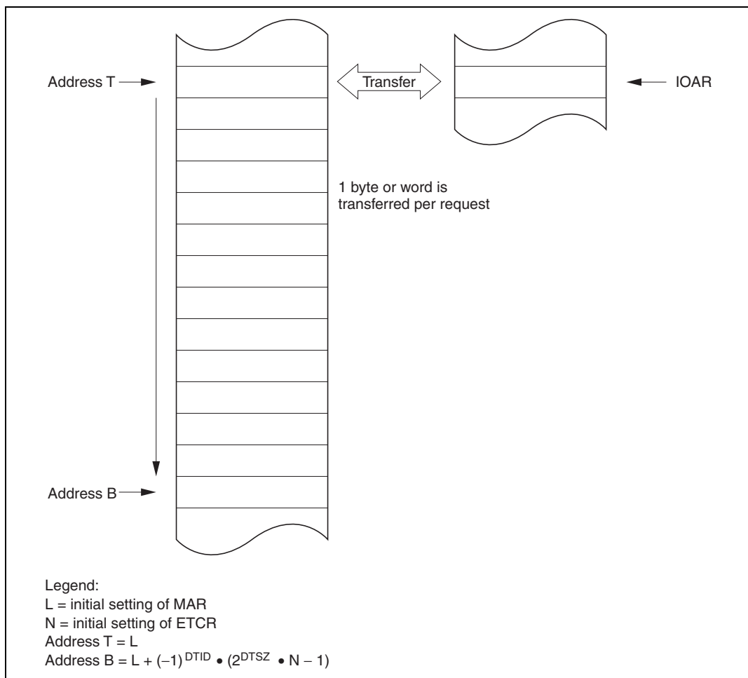
Figure 7.2 Operation in I/O Mode
