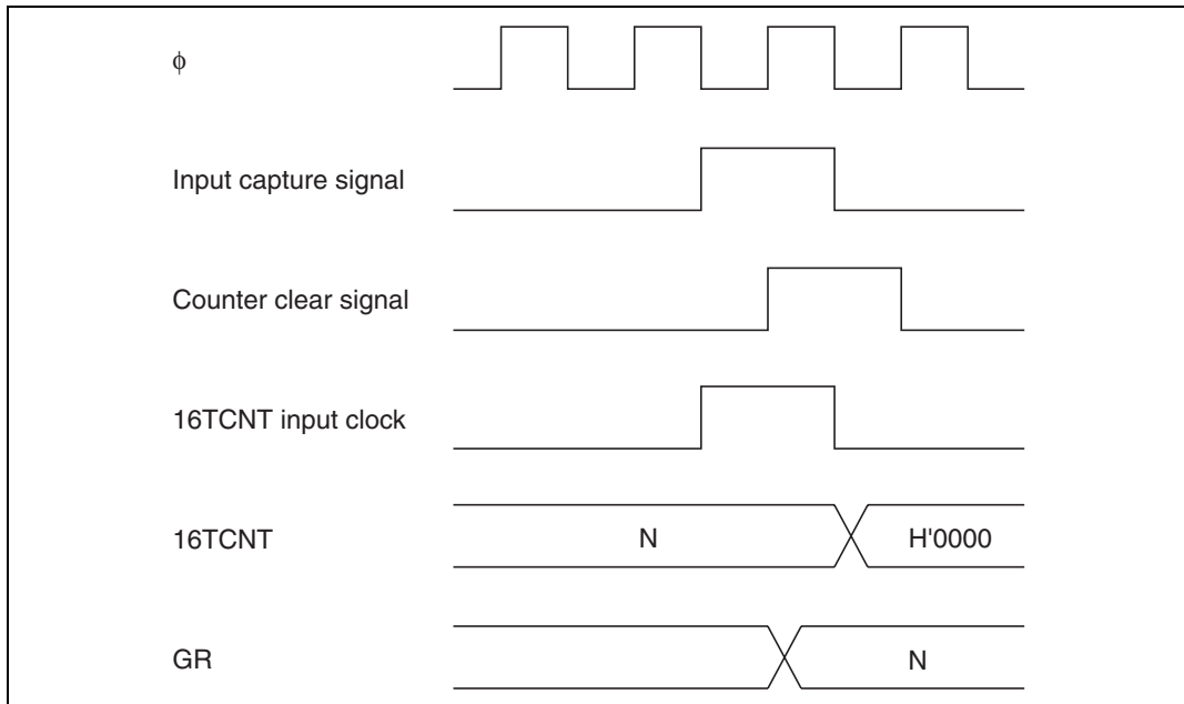
Figure 9.43 Contention between Counter Clearing by Input Capture and Counter Increment
