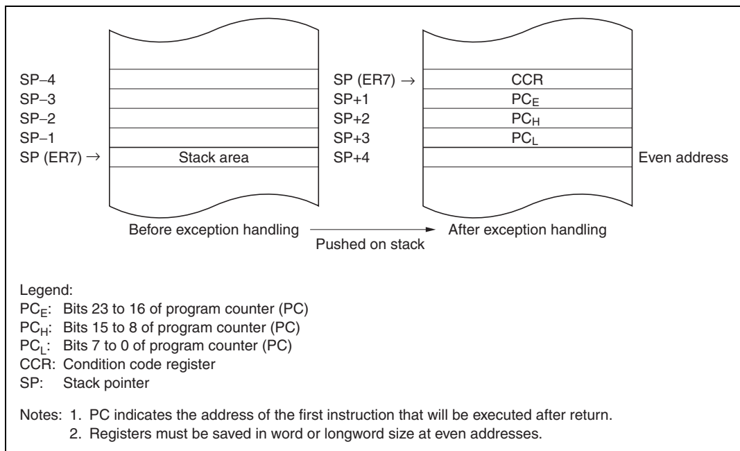
Figure 4.5 Stack after Completion of Exception Handling
