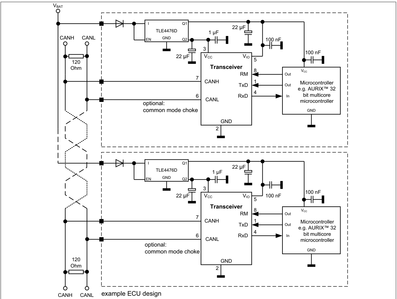
Figure 12 Application circuit
