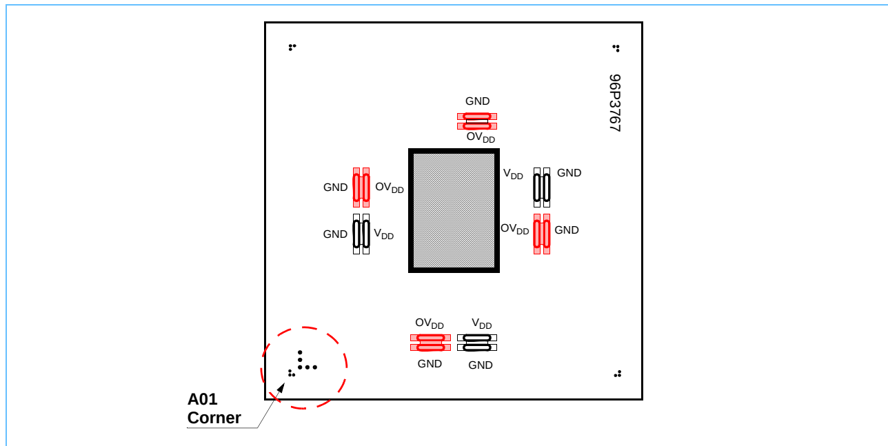
Figure 4-1. Module Substrate Decoupling Voltage Assignments
