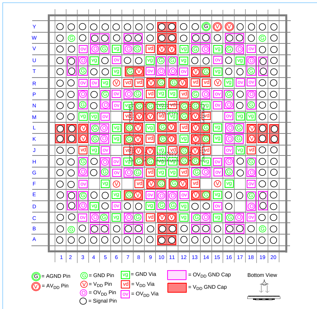
Figure 5-5. Orientation and Layout of the 750FL Microprocessor Decoupling Capacitors
