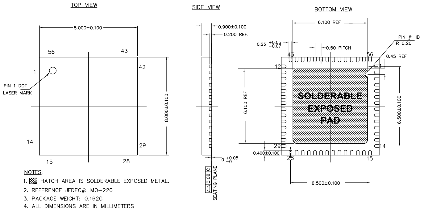
Figure 6. 56-pin QFN ( 8 \times 8 \times 1.0 \text{ mm} ) 6.1 \times 6.1 \text{ E-Pad (Sawn)} Package Outline, 51-85187
