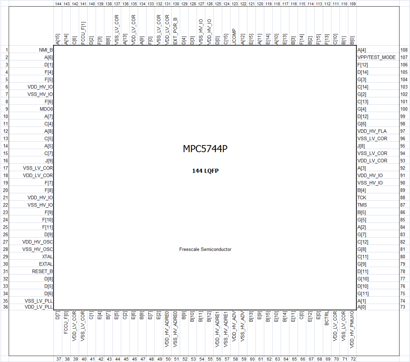
Figure 2. 144LQFP pinout
