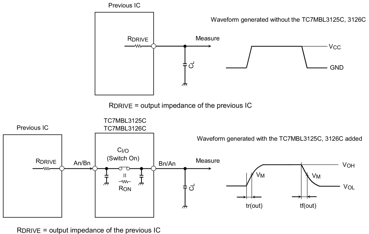
Fig. 12.1 Calculation Circuit
