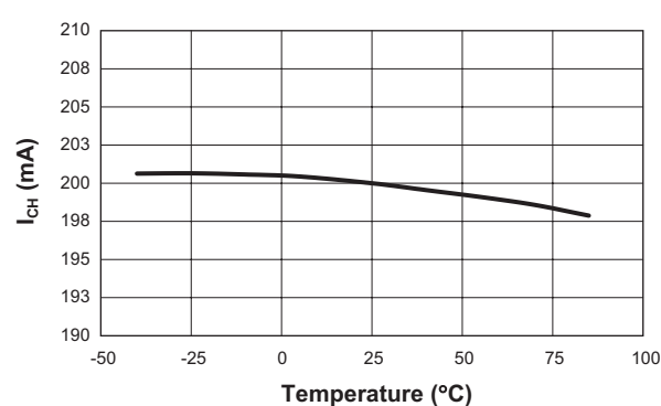
Constant Charging Current vs. Temperature ( R_{SET} = 8.06k\Omega )
