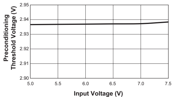
Preconditioning Voltage Threshold vs. Input Voltage (AAT3681A-4.1 and AAT3681A-5 Only)
