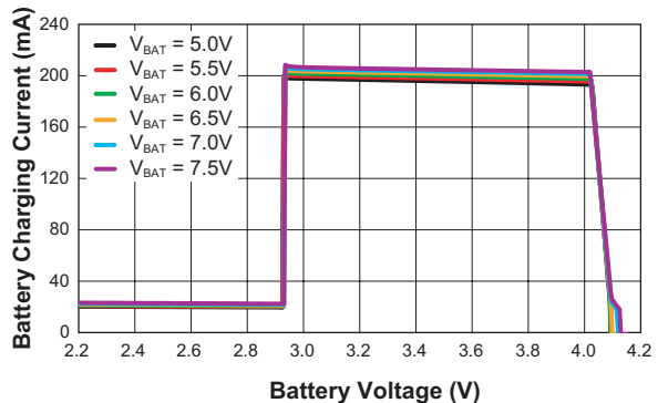
Battery Charging Current vs. Battery Voltage (AAT3681A-4.1 and AAT3681A-5 Only)
