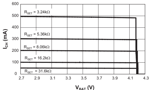
Charging Current vs. Battery Voltage (AAT3681A-1 and AAT3681A-4 only)
